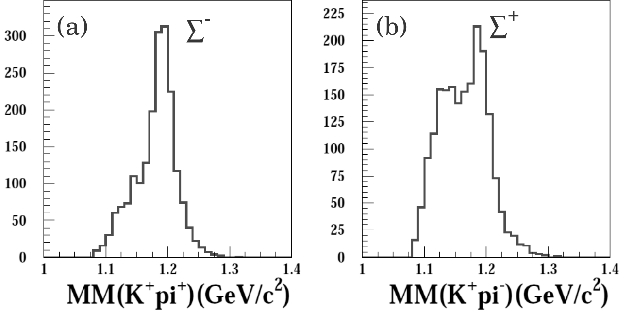
Figure 3.18: The distributions of MM(K^+\pi) for events which survived the neutron selection cut and the \pi^0 rejection cut. (a) MM(K^+\pi^+) , (b) MM(K^+\pi^-) .
