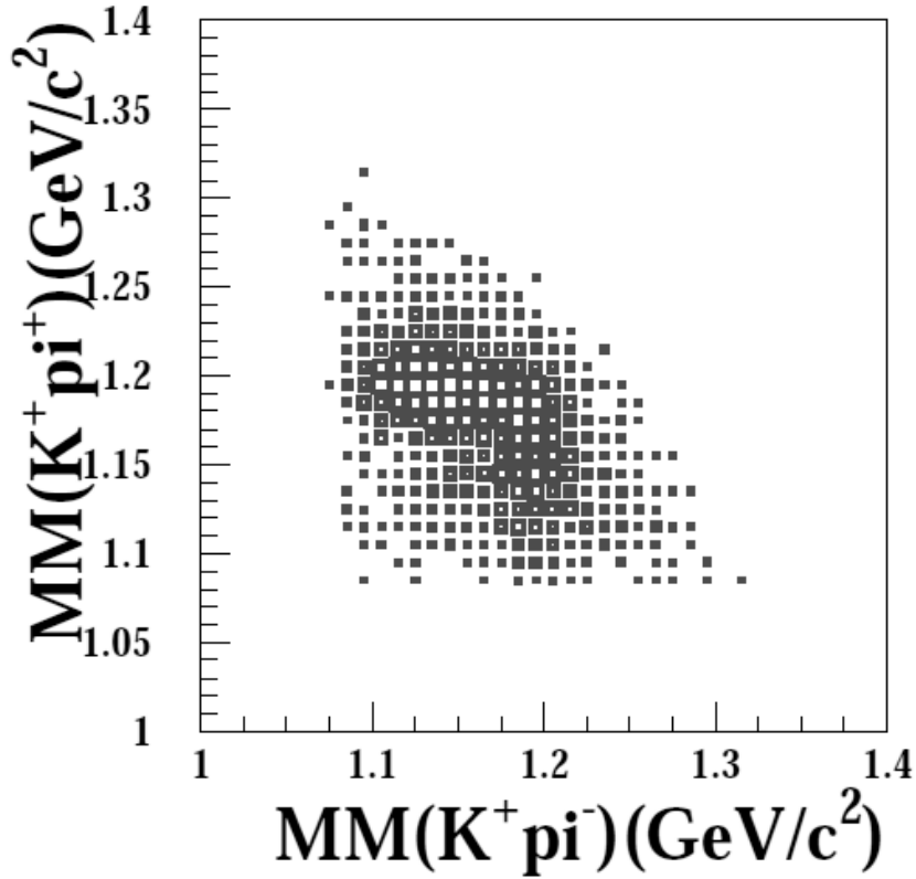
Figure 3.19: The correlation between MM(K^+\pi^+) and MM(K^+\pi^-) .
