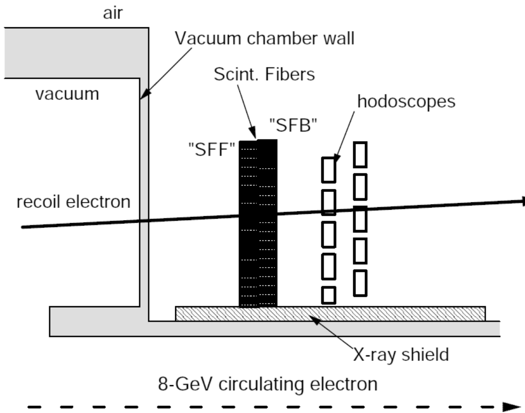
Figure 2.10: Schematic view of the tagging system
