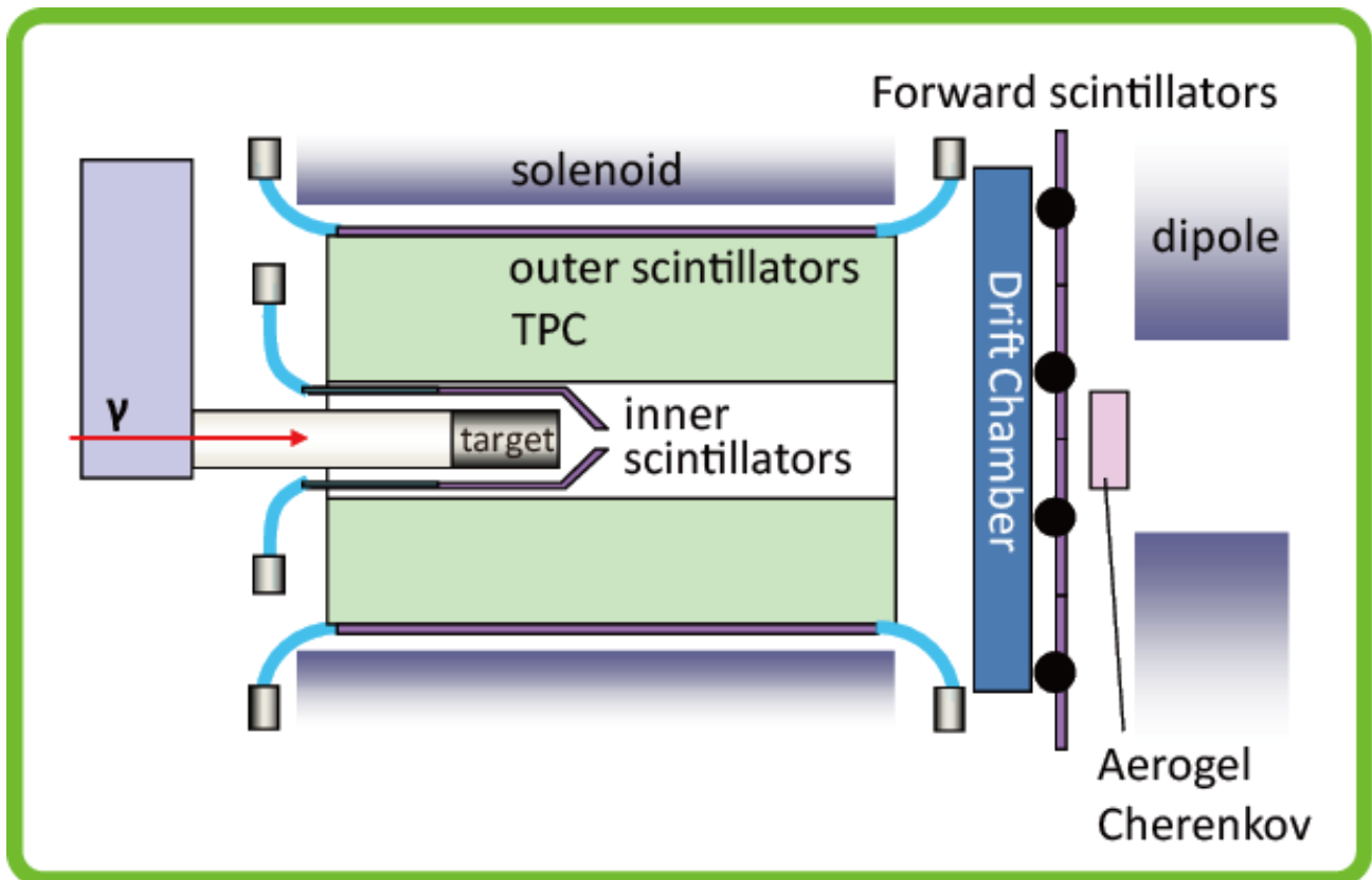
Figure 2.18: Inner scintillation counters and outer counters
