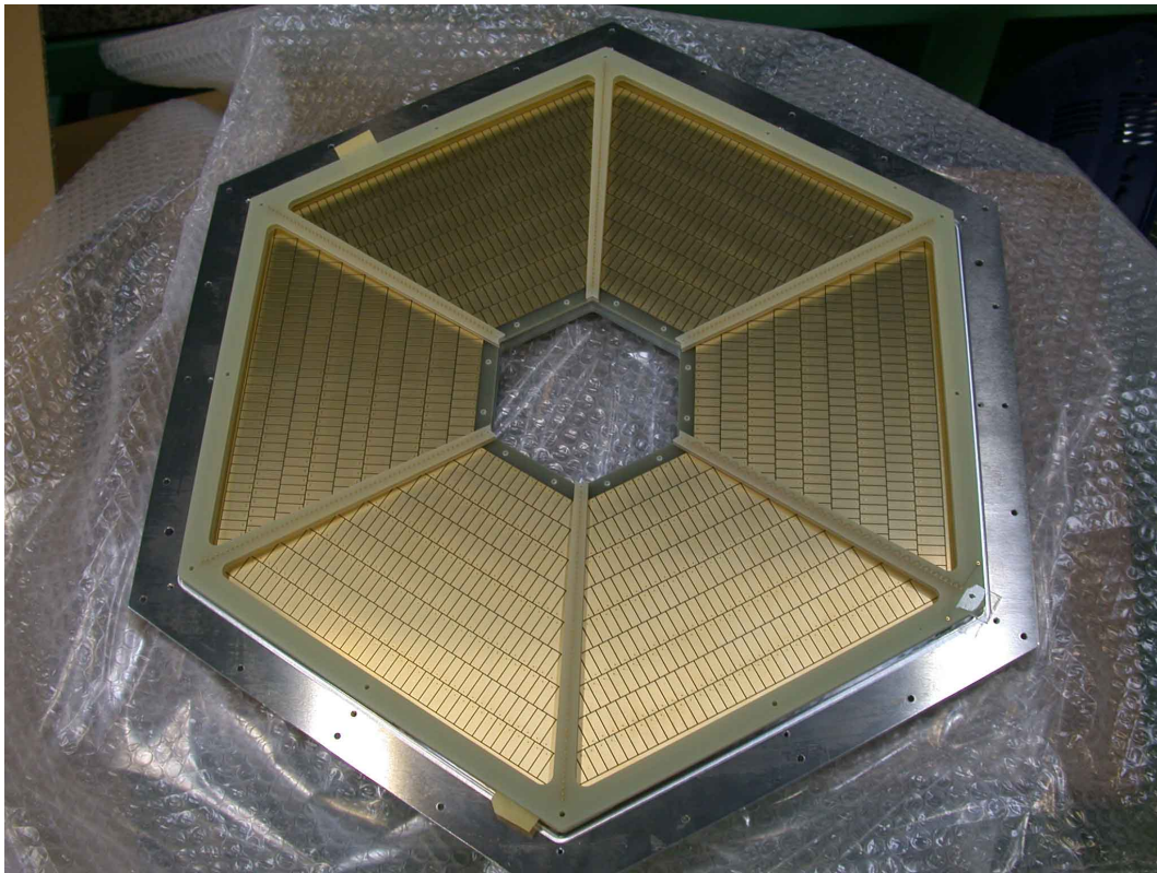
Figure 2.33: Picture of the pad plane of the TPC.
