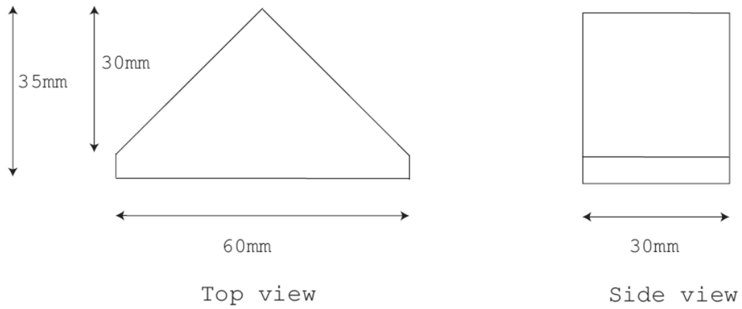
Figure 2.8: Schematic view of the prism
