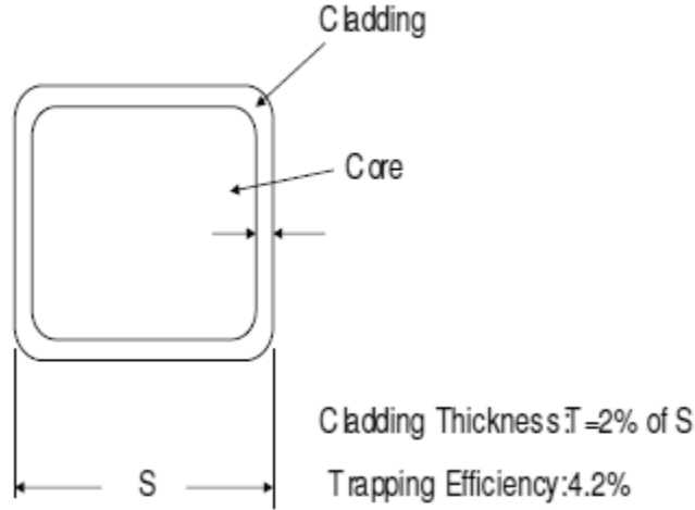
Figure 2.11: Schematic view of the fiber
