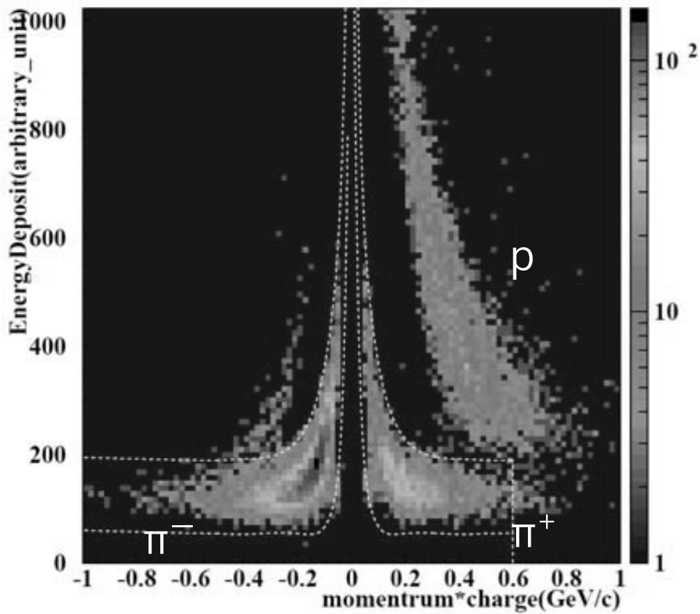
Figure 3.7: Correlation between the momentum and energy deposit in the TPC. The x and y axes represent the momentum \times charge and the energy deposit of a track, respectively. The loci of p , \pi^+ and \pi^- can be seen clearly. The K^- locus is also seen in the negative charge region. The K^+ can not be seen because a K^+ is identified in the forward spectrometer for events in this plot.
