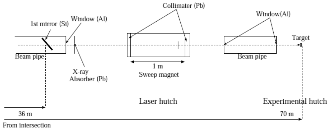
Figure 2.12: Schematic view of the LEPS beam line setup.
