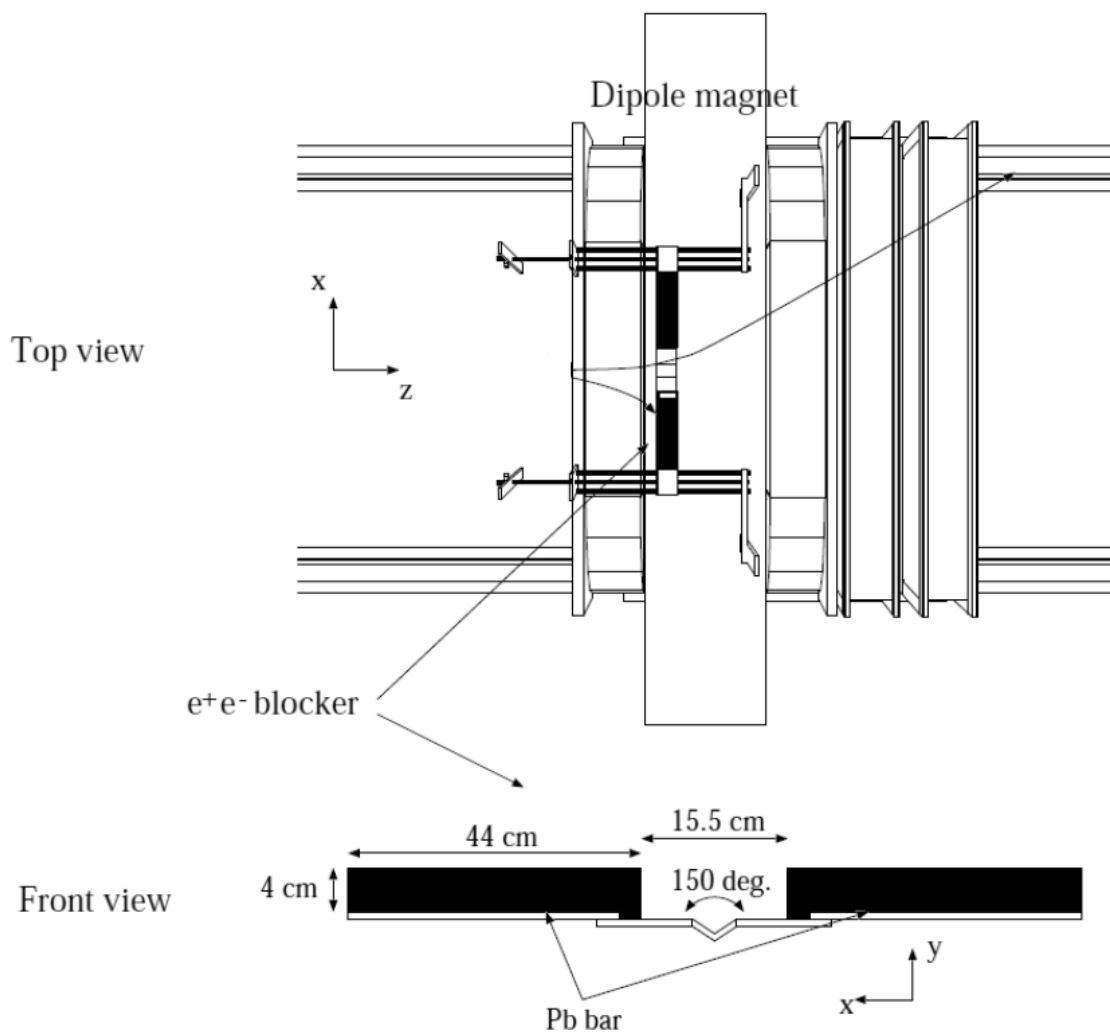
Figure 2.19: Drawing of the e^+e^- blocker.
