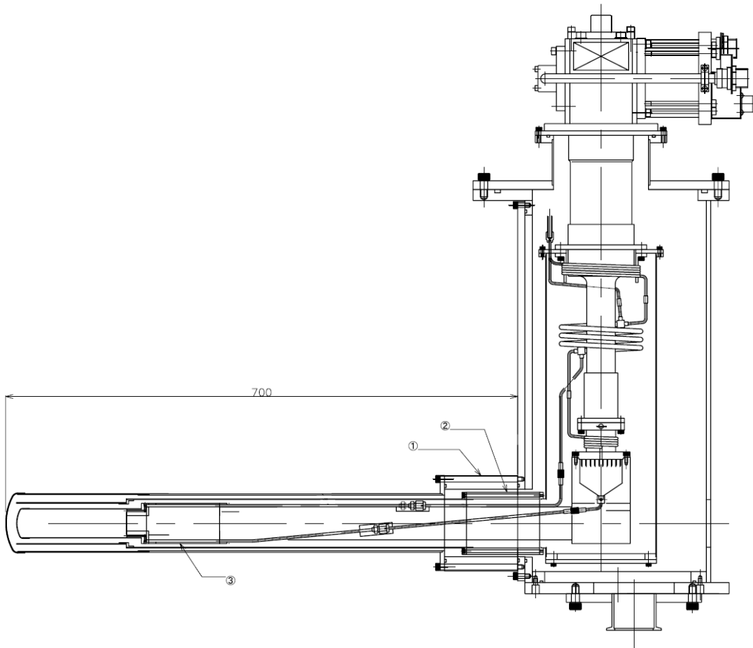
Figure 2.25: A schematic view of the liquid target system.
