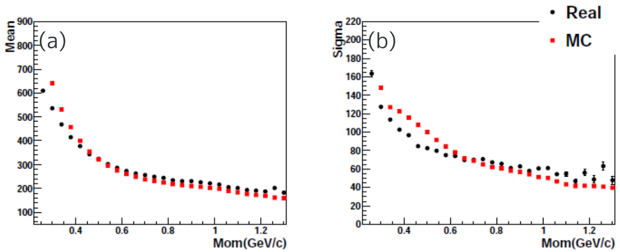
Figure 3.6: (a) The most probable value and (b) \sigma of dE/dx of \pi^- tracks as a function of momentum. Black and red circles correspond to the real data and Monte Carlo simulation, respectively.
