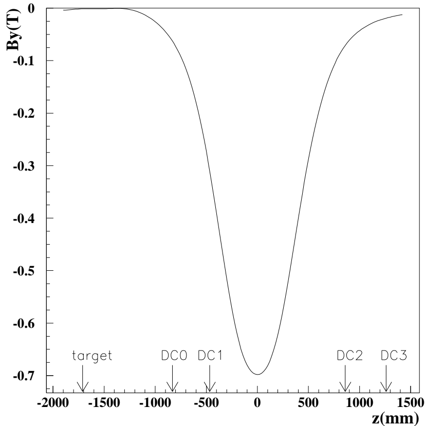
Figure 2.22: Distribution of the magnetic field B_y as a function of the z -position at x=0 and y=0 . The position of z=0 corresponds to the center of the dipole magnet.
