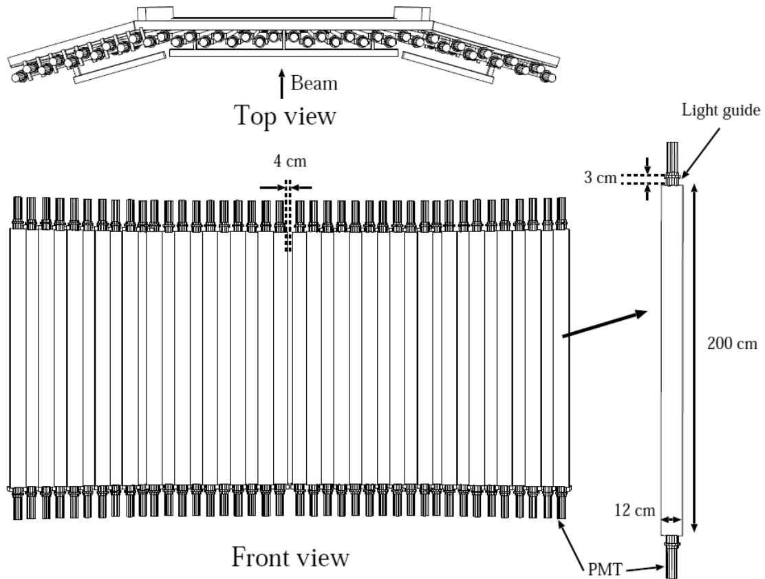
Figure 2.21: Drawing of the TOF wall.
