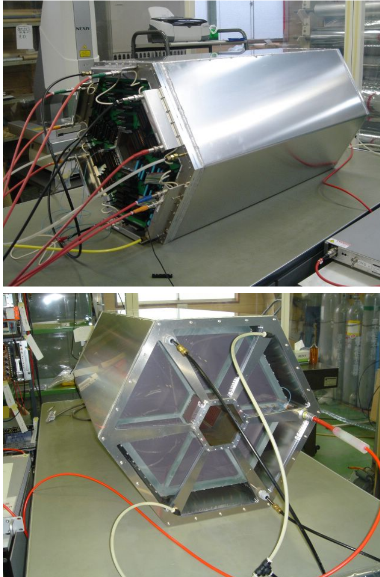
Figure 2.30: The overall views of the Time Projection Chamber. The top and down pictures show upstream and downstream side of the TPC, respectively.
