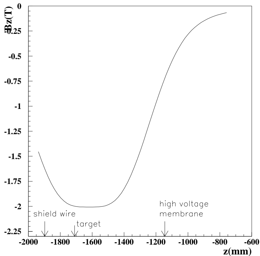
Figure 2.23: Distribution of the z-component of the solenoid magnetic field B_z as a function of the z-coordinate on the beam axis ( x=0,y=0 ).
