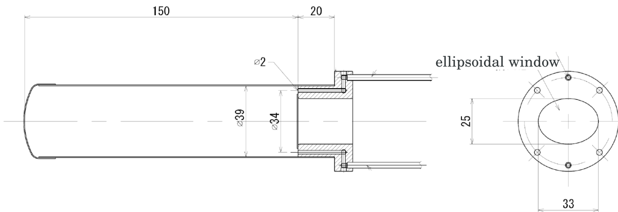
Figure 2.26: A schematic view of the target cell.
