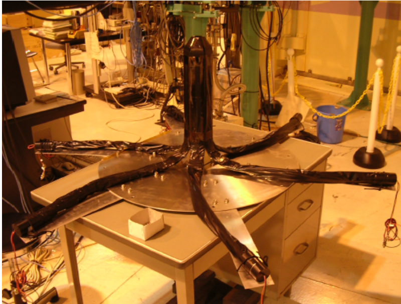
Figure 2.16: Picture of combined inner scintillation counters.
