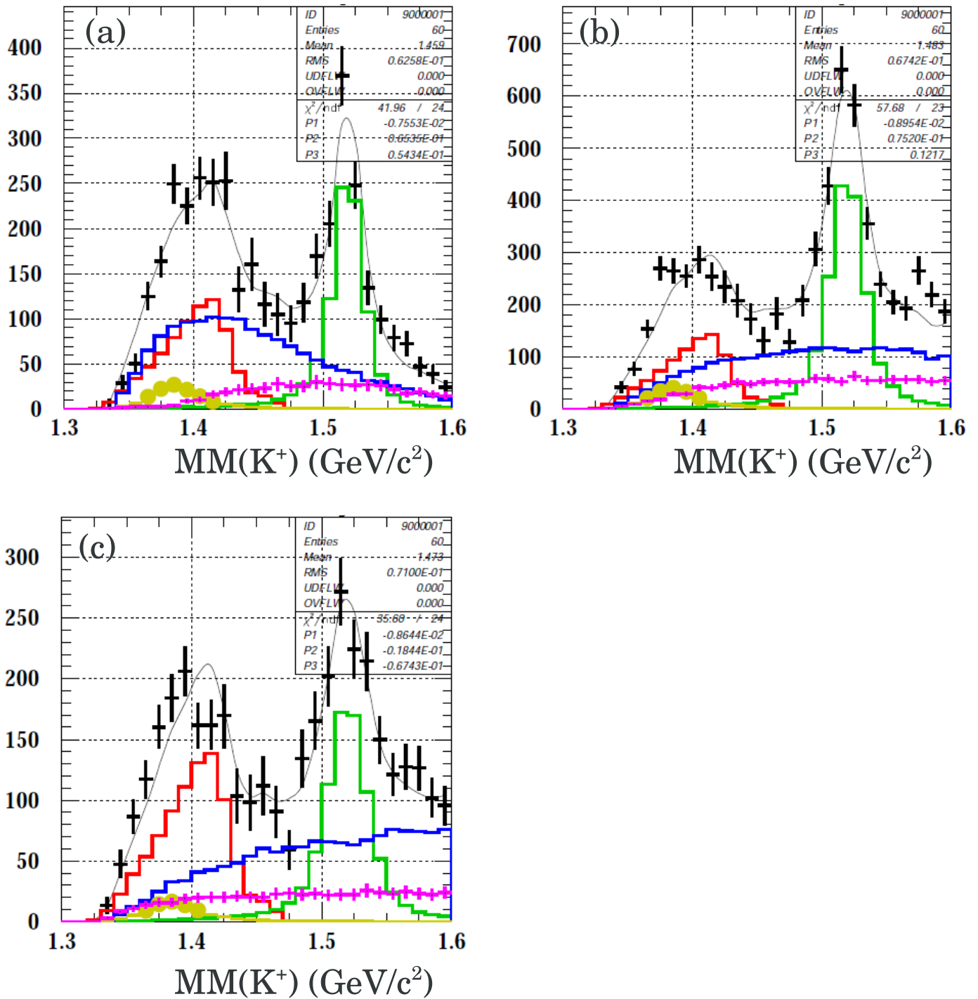
Figure 3.23: The combined MM(K^+) spectrum. The solid line, black, red, yellow, blue, green, magenta plot show the fitted result, data, the mass spectra of \Lambda(1405) calculated by Nacher et al. , \Sigma^0(1385) , nonresonant K^+\Sigma\pi , \Lambda(1520) and K^0(892)\Sigma^+ , respectively.
