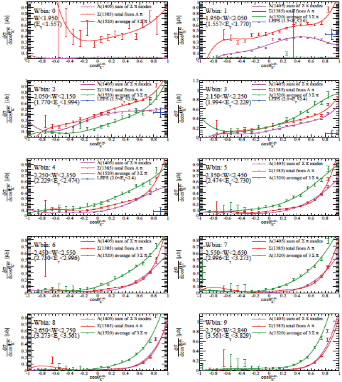
Figure 1.7: Differential cross sections for \Sigma^0(1385) (red), \Lambda(1405) (magenta) and \Lambda(1520) (green) photoproduction measured at CLAS.
