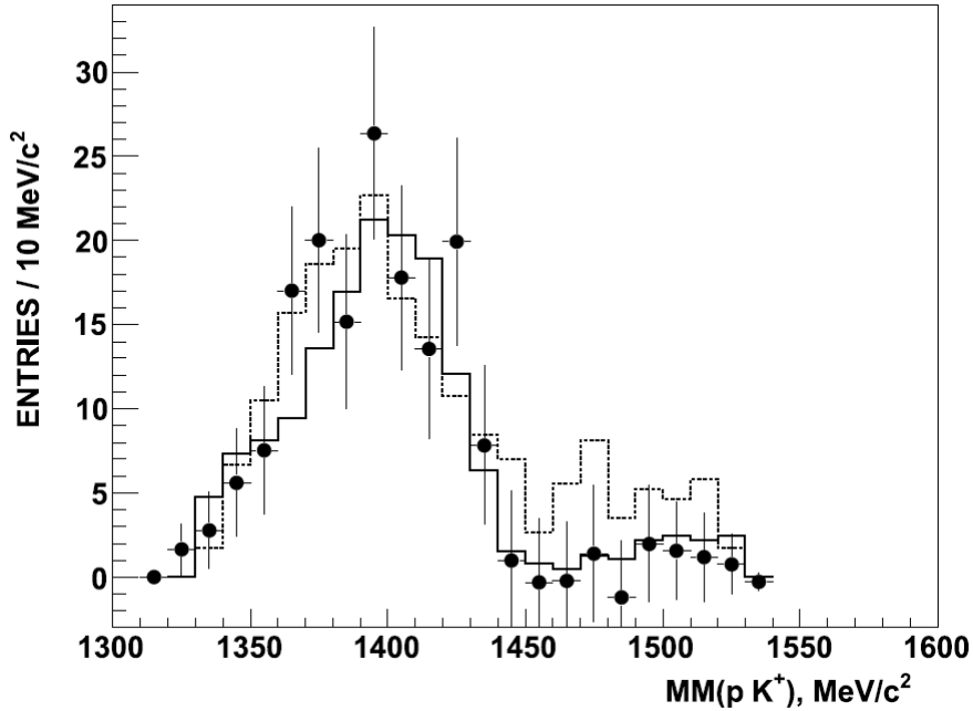
Figure 1.3: The invariant mass spectrum of the \Lambda(1405) . The spectrum measured by Zychor et al. is shown by closed circles. The spectra obtained by Hemingway and Thomas et al. are shown by the solid and dashed histograms, respectively. The solid and dashed histograms are normalized to the height of the spectrum measured by Zychor et al.
