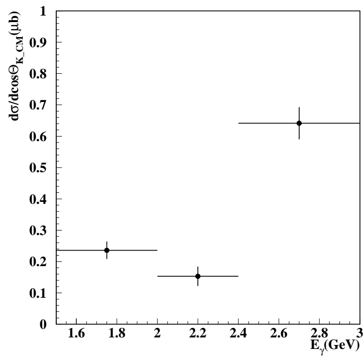
Figure 4.2: The photon energy dependence of the differential cross section of \gamma p \rightarrow K^+ \Lambda(1405) reaction.
