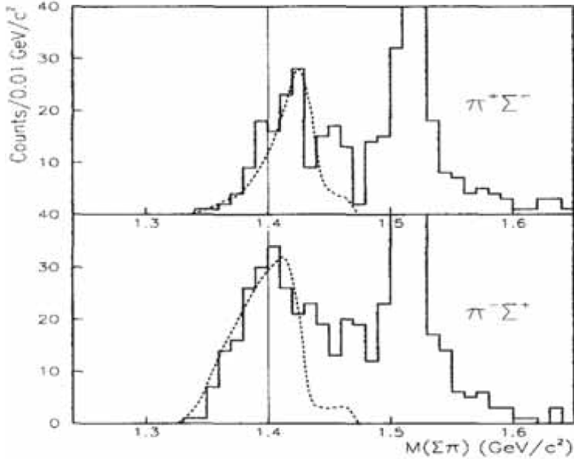
Figure 1.4: Invariant mass spectra of the \Lambda(1405) measured by J.K.Ahn at LEPS [21]. The theoretical spectra by Nacher et al. [9] are shown as the dotted lines.
