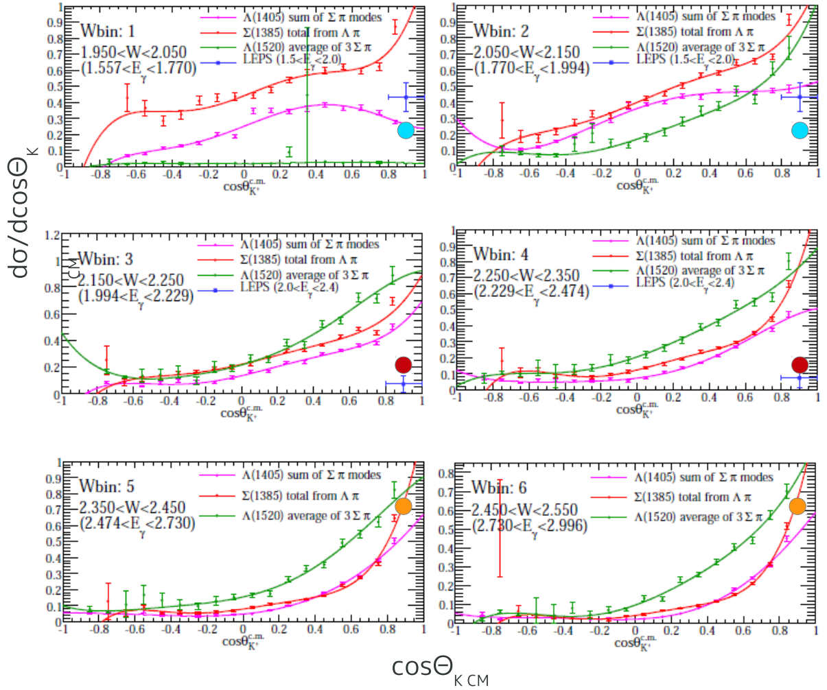
Figure 4.7: Comparison of the differential cross section for \Lambda(1405) between CLAS and this analysis. Magenta line shows the \Lambda(1405) result of CLAS. Blue, red and yellow points correspond to this analysis in the E_\gamma region of 1.5 < E_\gamma < 2.0 GeV, 2.0 < E_\gamma < 2.4 GeV and 2.4 < E_\gamma < 3.0 GeV, respectively.
