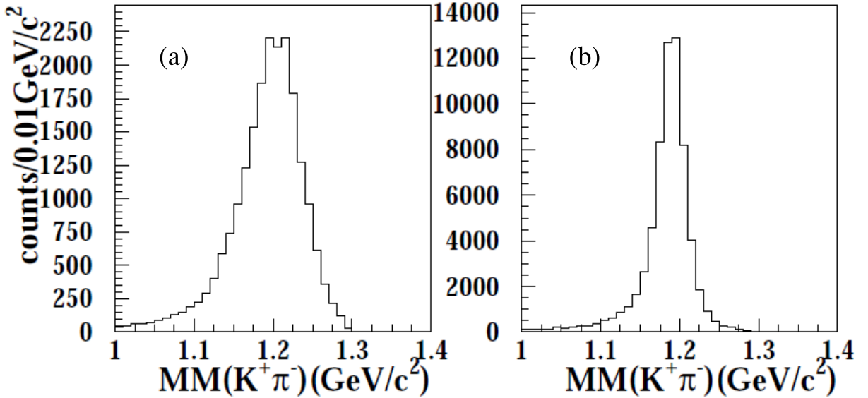
Figure 3.11: Distributions of MM(K^+\pi^-) obtained by the Monte-Carlo simulation of the \gamma p \rightarrow K^+\Sigma^0(1385) \rightarrow K^+\Lambda\pi^0 \rightarrow K^+p\pi^-\pi^0 and \gamma p \rightarrow K^+\Lambda(1405) \rightarrow K^+\Sigma^+\pi^- \rightarrow K^+p\pi^0\pi^- reactions. MM(K^+\pi^-) distributions for \Sigma^0(1385) and \Lambda(1405) are shown in (a) and (b), respectively.
