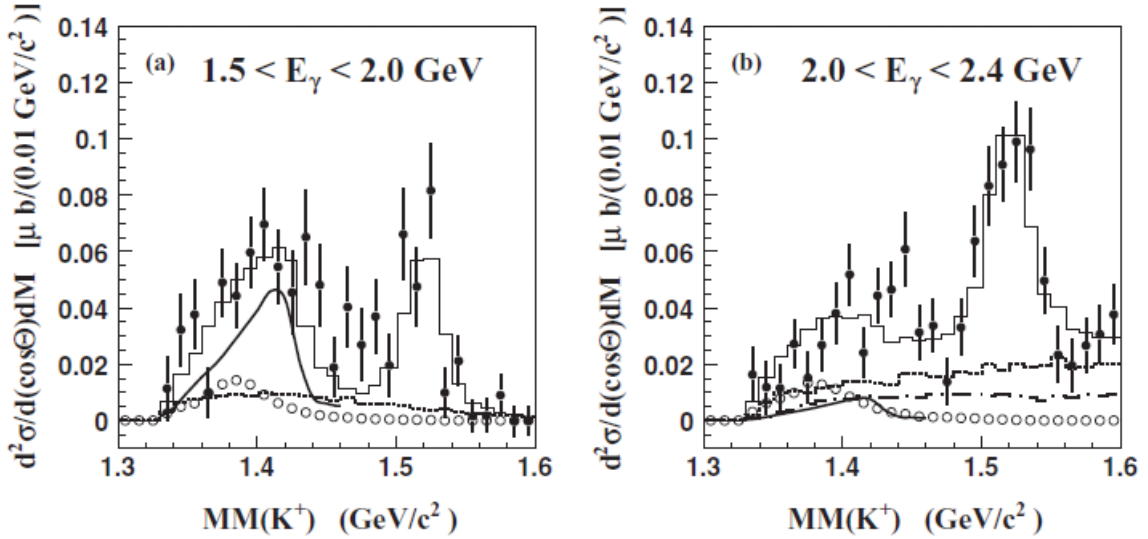
Figure 1.6: The missing mass spectra of the reaction \gamma p \rightarrow K^+ X ( MM(K^+) ) obtained by Niijima et al. . The spectra are shown in two photon energy ranges: (a) 1.5 < E_\gamma < 2.0 GeV and (b) 2.0 < E_\gamma < 2.4 GeV.
