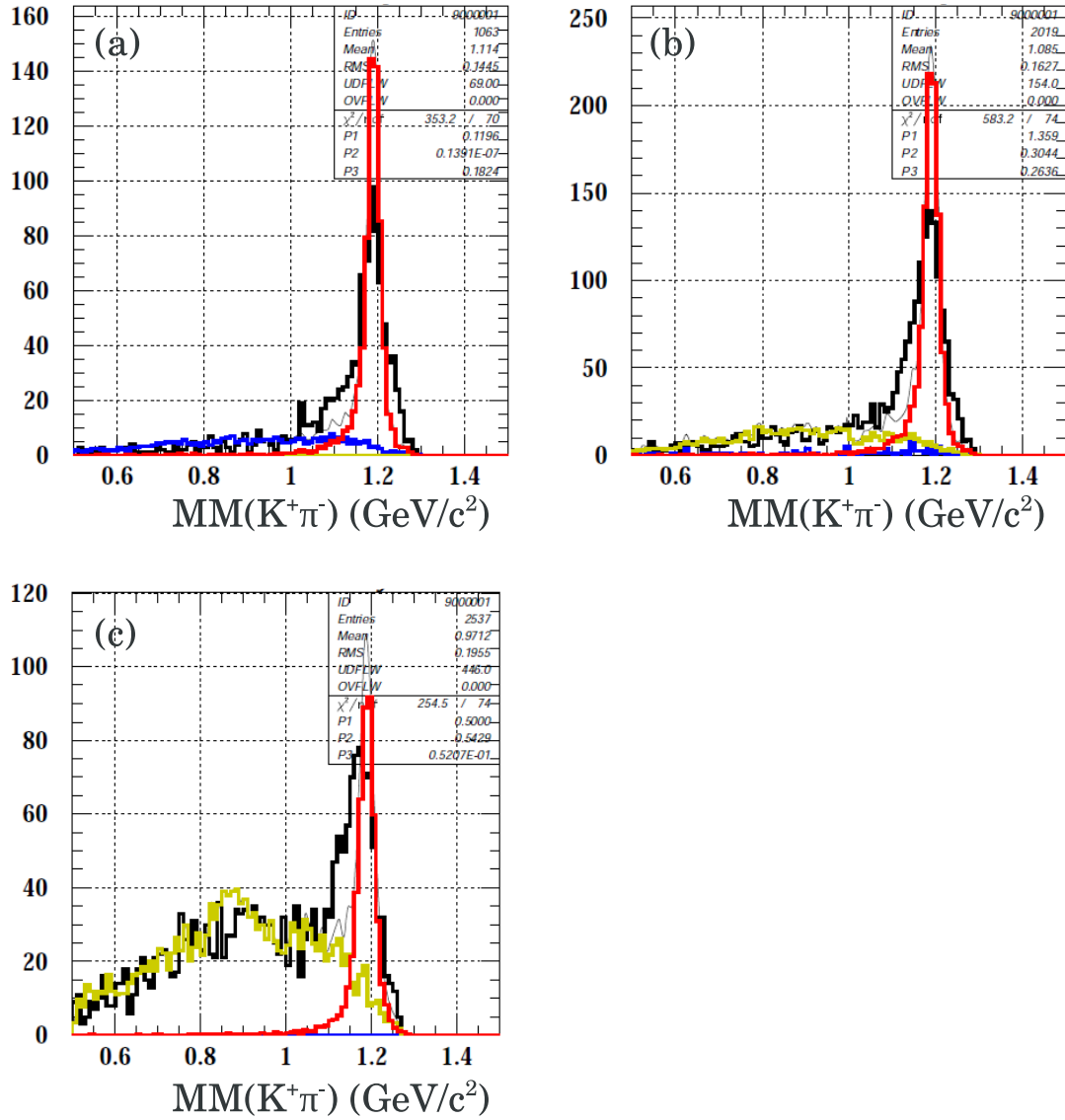
Figure 3.14: Distribution of the MM(K^+\pi^-) after the \Lambda rejection cut and the cut of 1.3 < MM(K^+) < 1.45 \text{GeV}/c^2 in three photon energy ranges: (a) 1.5 < E_\gamma < 2.0 \text{GeV} , (b) 2.0 < E_\gamma < 2.4 \text{GeV} and (c) 2.4 < E_\gamma < 3.0 \text{GeV} .
