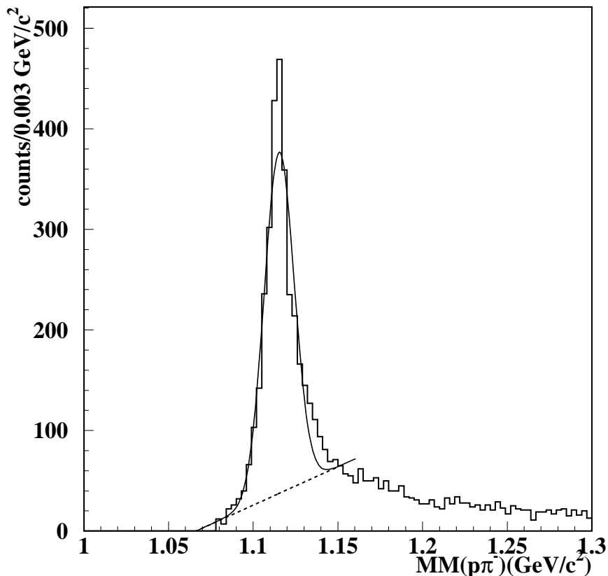
Figure 3.8: Invariant mass spectra of p\pi^- pairs.
