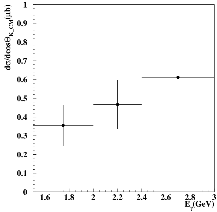
Figure 4.1: The photon energy dependence of the differential cross section of \gamma p \rightarrow K^+ \Sigma^0(1385) reaction.
