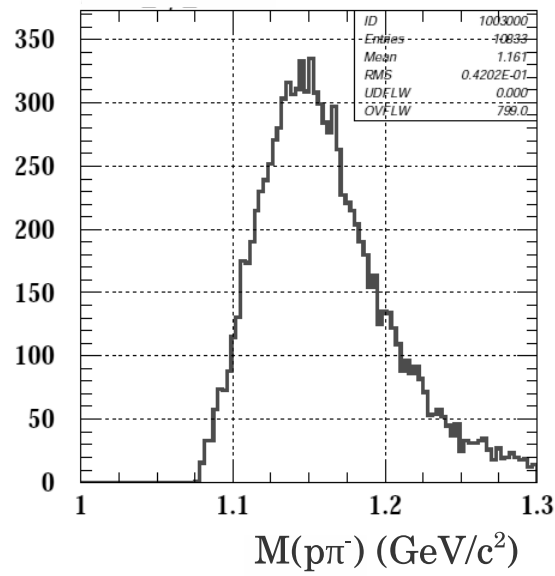
Figure 3.13: Distribution of the invariant mass of p\pi^- pairs ( M(p\pi^-) ) obtained by the Monte-Carlo simulation of \Lambda(1405) photoproduction.
