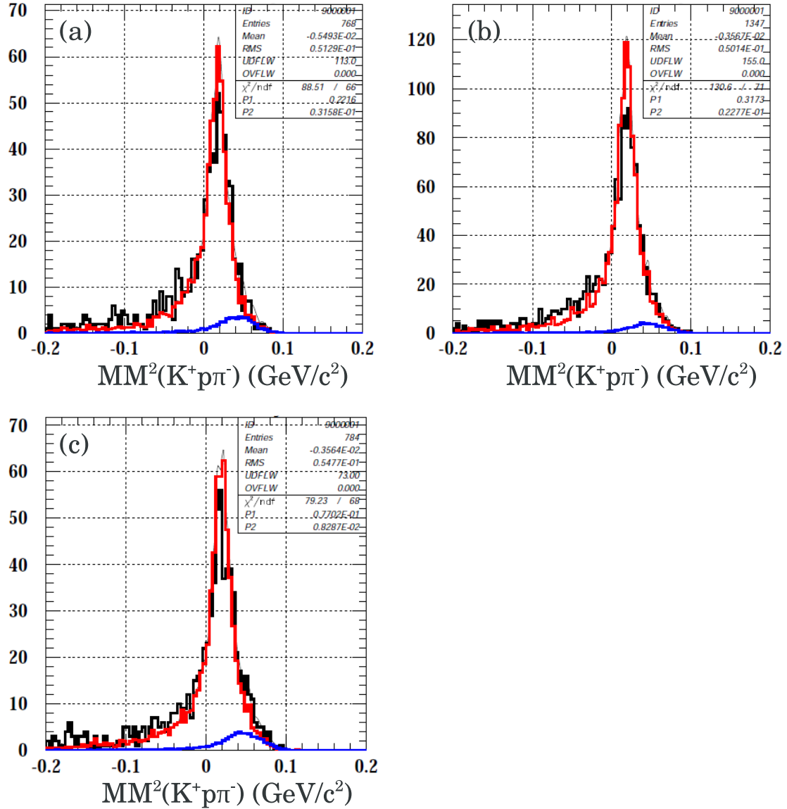
Figure 3.10: Distribution of the MM^2(K^+ p \pi^-) after the \Lambda selection cut and the cut of 1.3 < MM(K^+) < 1.45 \text{GeV}/c^2 in three photon energy ranges: 1.5 < E_\gamma < 2.0 \text{GeV} , 2.0 < E_\gamma < 2.4 \text{GeV} and 2.4 < E_\gamma < 3.0 \text{GeV} . The black histogram shows real data. The red and blue histogram show the shape of Monte Carlo simulation for \gamma p \rightarrow K^+ \Sigma^0(1385) \rightarrow K^+ \Lambda \pi^0 and \gamma p \rightarrow K^+ \Lambda(1405) \rightarrow K^+ \Sigma^0 \pi^0 \rightarrow K^+ \Lambda \gamma \pi^0 , respectively.
