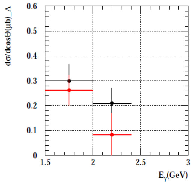
Figure 4.5: Comparison of the differential cross section for \Lambda(1405) between Niyama et al. and this analysis, after normalized to D.S.Ahn. Red and black points correspond to the data of Niyama and this analysis, respectively.
