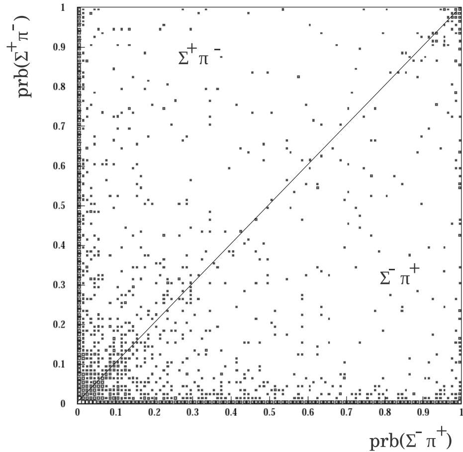
Figure 3.21: The correlation of the \chi^2 probability of the kinematic fit between the \Sigma^- \pi^+ assumption ( \text{prob}_{\Sigma^- \pi^+} ) and the \Sigma^+ \pi^- assumption ( \text{prob}_{\Sigma^+ \pi^-} ).
