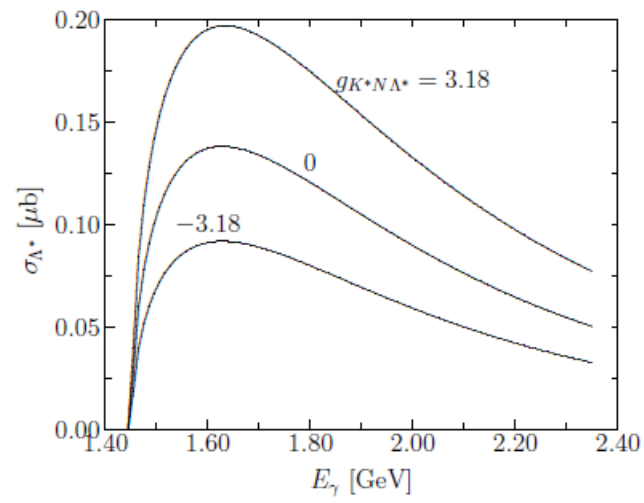
Figure 1.8: The total cross section for \Lambda(1405) photoproduction calculated by Nam et al. [27].
