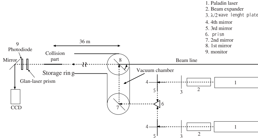
Figure 2.6: Schematic view of the laser operating system
