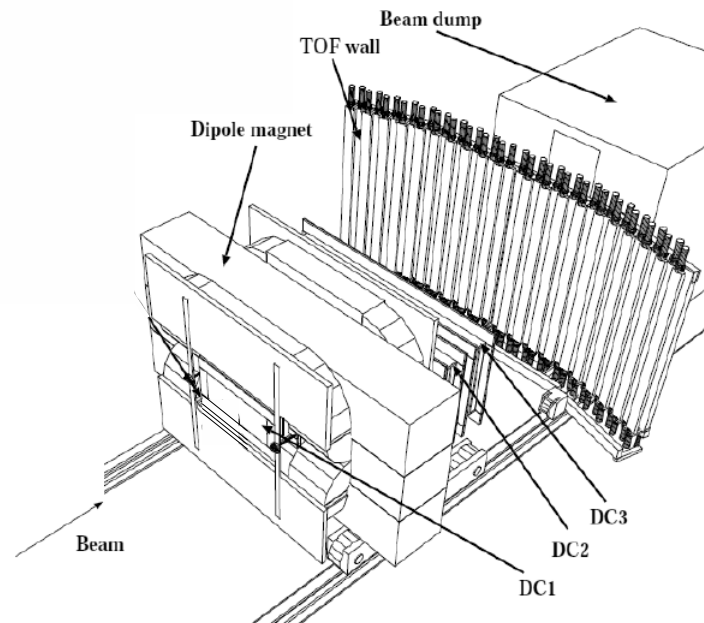
Figure 2.14: Overview of the LEPS spectrometer.
