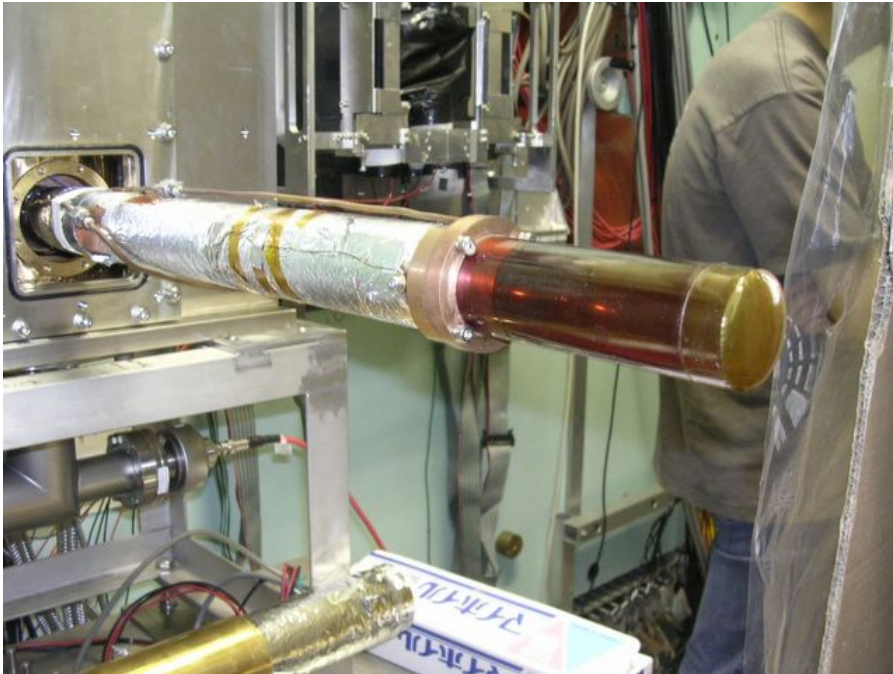
Figure 2.28: Picture of the target cell.
