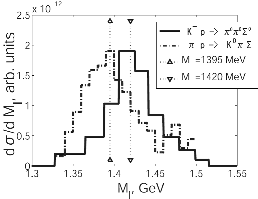
Figure 1.2: Mass spectra of the \Lambda(1405) measured by Prakhov et al. (solid) and Thomas et al. (dashed). The triangles indicate the mass peak position of the \Lambda(1405) calculated by Magas et al.
