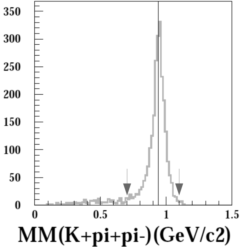
Figure 3.16: Distribution of the missing mass of the \gamma p \rightarrow K^+ \pi^+ \pi^- X reaction, MM(K^+ \pi^+ \pi^-) .
