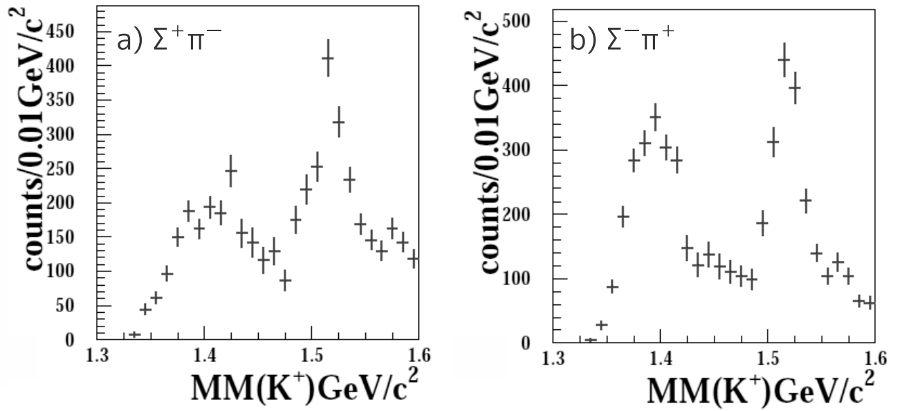
Figure 3.22: The missing mass distribution for the \gamma p \rightarrow K^+ X reaction for (a) the K^+ \Sigma^+ \pi^- final state and (b) K^+ \Sigma^- \pi^+ final state.
