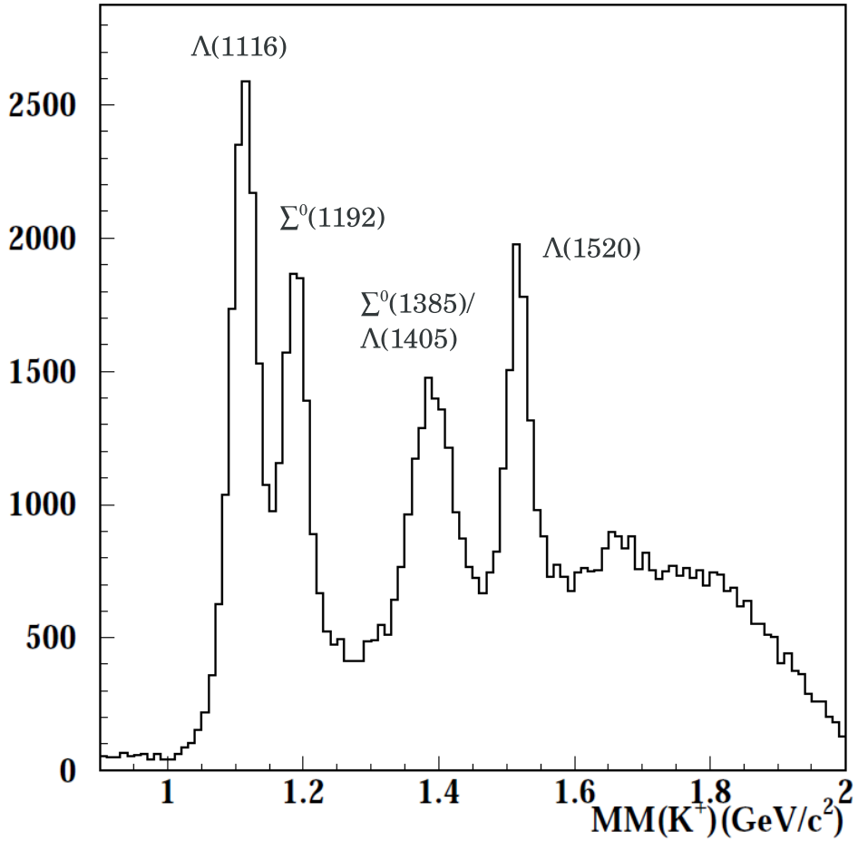
Figure 3.4: The missing mass distribution of \gamma p \rightarrow K^+ X reaction
