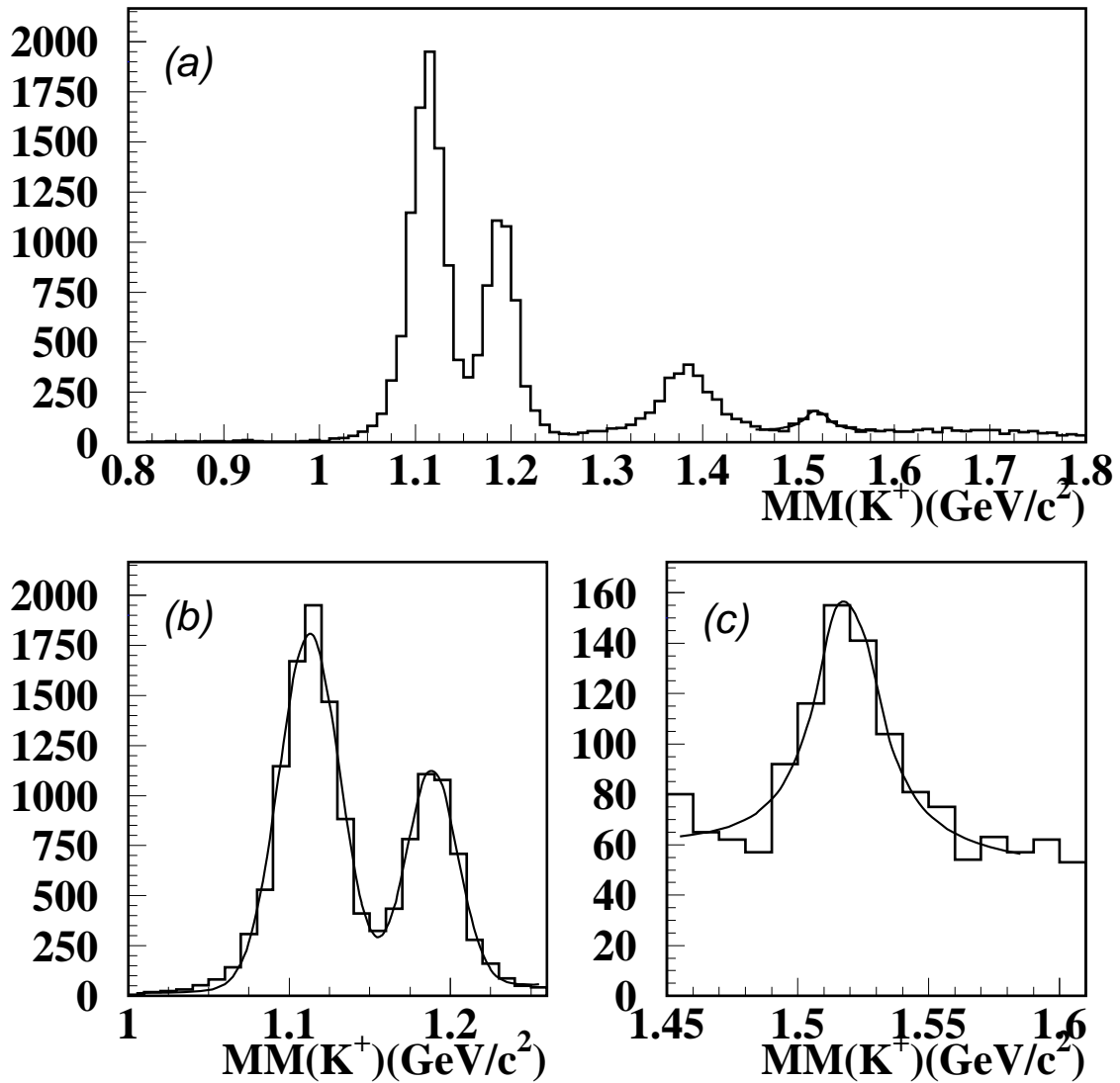
Figure 3.9: Missing mass of the \gamma p \rightarrow K^+ X reaction after the \Lambda selection cut for all E_\gamma range: 1.5 < E_\gamma < 3.0 GeV. (a) whole MM(K^+) range, (b) around \Lambda and \Sigma^0 and (c) around \Lambda(1520) .
