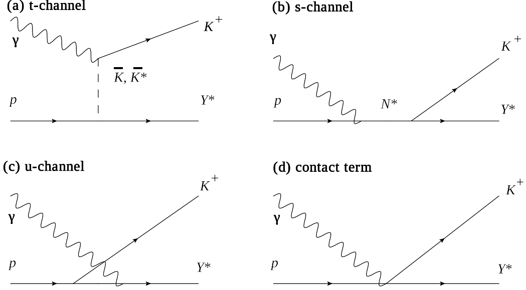
Figure 1.5: Feynman diagrams for the \gamma p \rightarrow K^+ Y^* reaction.
