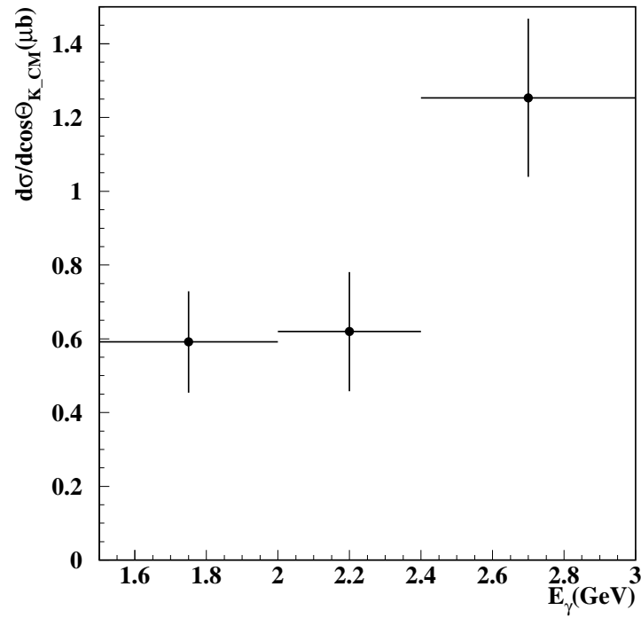
Figure 4.3: The photon energy dependence of the sum of the differential cross section of \gamma p \rightarrow K^+ \Lambda(1405) reaction and \gamma p \rightarrow K^+ \Sigma^0(1385) reaction.
