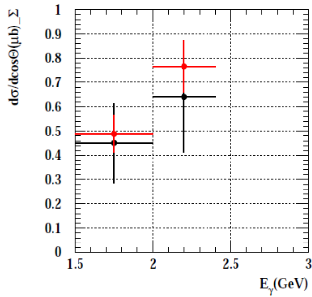
Figure 4.6: Comparison of the differential cross section for \Sigma^0(1385) between Niyama et al. and this analysis, after normalized to D.S.Ahn. Red and black points correspond to the data of Niyama and this analysis, respectively.
