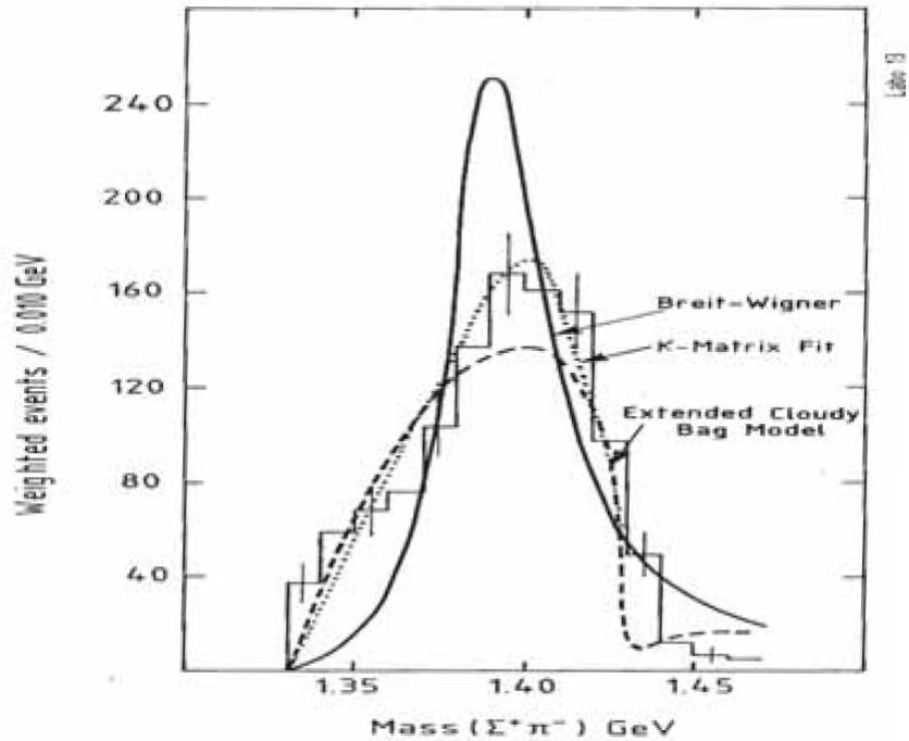
Figure 1.1: Invariant mass spectrum of the \Lambda(1405) measured by Hemingway via the K^- p \rightarrow \pi^- \pi^+ \Lambda(1405) reaction.
