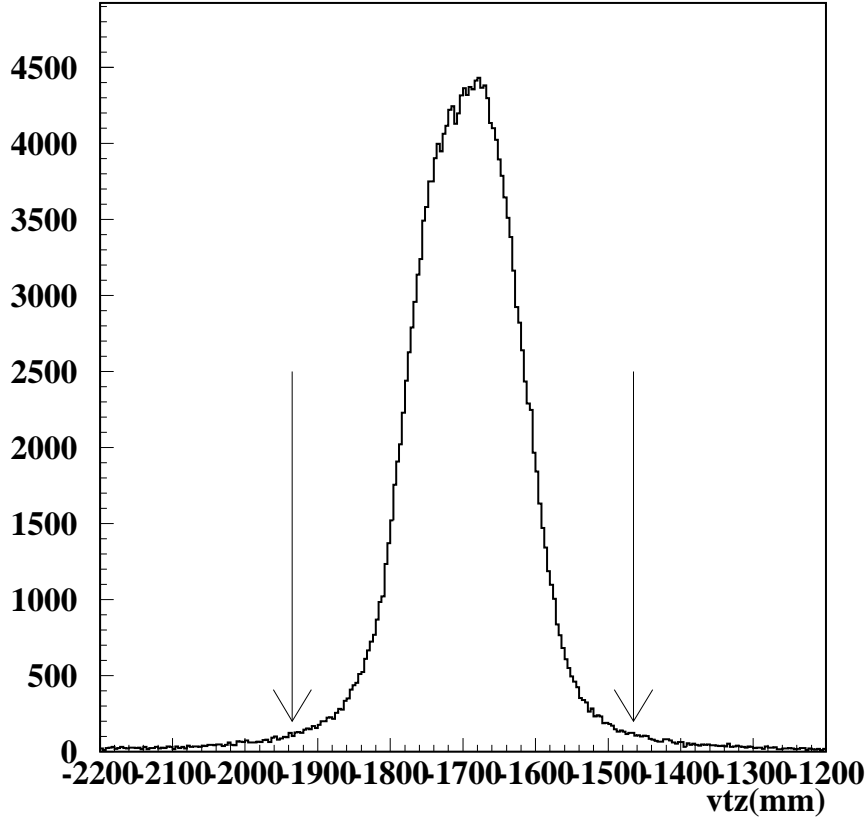
Figure 3.3: The distribution of z coordinate of the closest point between a K^+ track and the beam axis.
