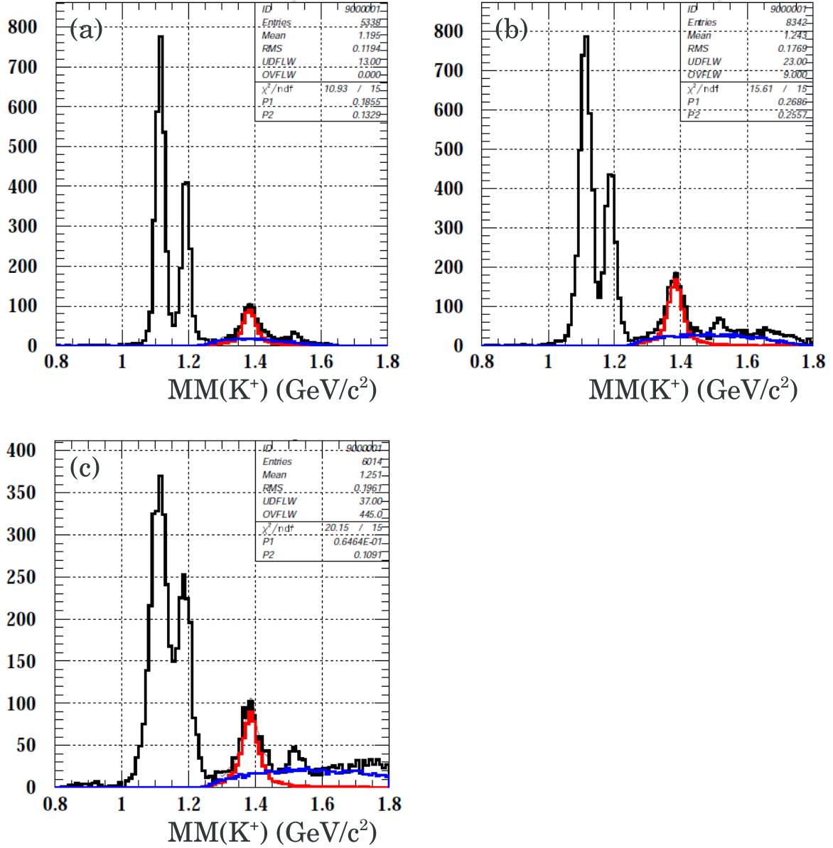
Figure 3.15: Missing mass of the \gamma p \rightarrow K^+ X reaction after the \Lambda selection cut at each E_\gamma region: (a) 1.5 < E_\gamma < 2.0 GeV, (b) 2.0 < E_\gamma < 2.4 GeV, (c) 2.4 < E_\gamma < 3.0 GeV. Black, red and blue histograms represent the real data, MC of \Sigma^0(1385) and MC of non-resonant \Lambda\pi^0 .
