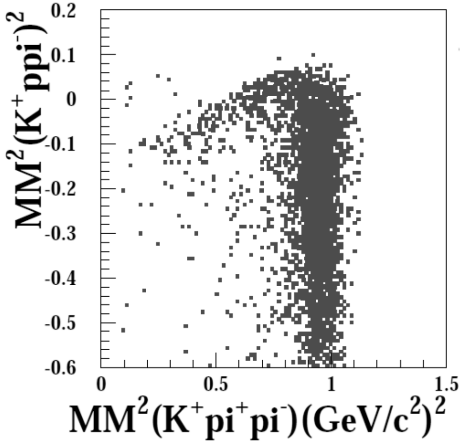
Figure 3.17: A correlation plot between the MM(K^+\pi^+\pi^-) and the MM^2(K^+p\pi^-) .
