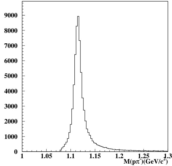
Figure 3.12: Distribution of the invariant mass of p\pi^- pairs ( M(p\pi^-) ) obtained by the Monte-Carlo simulation of \Sigma^0(1385) photoproduction.
