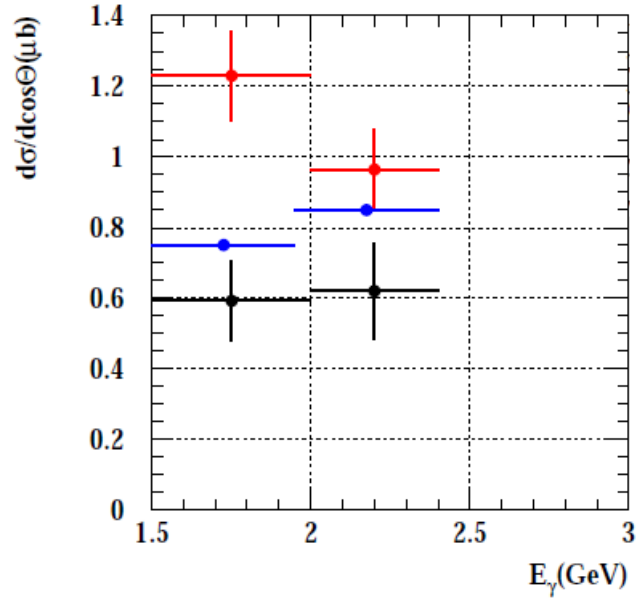
Figure 4.4: Comparison of the sum of the differential cross section for \Lambda(1405) and \Sigma^0(1385) between D.S.Ahn, Niyama et al. and this analysis. Blue, red and black points correspond to the data of D.S.Ahn, Niyama and this analysis, respectively.
