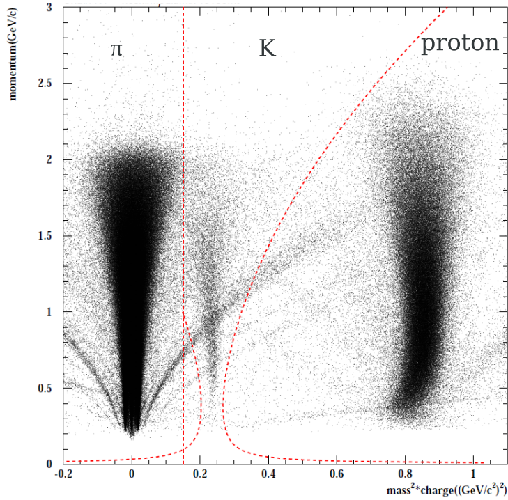
Figure 3.1: Scatter plot of the momentum and reconstructed mass of particles at forward spectrometer. Dashed lines show K^+ selection boundary.
