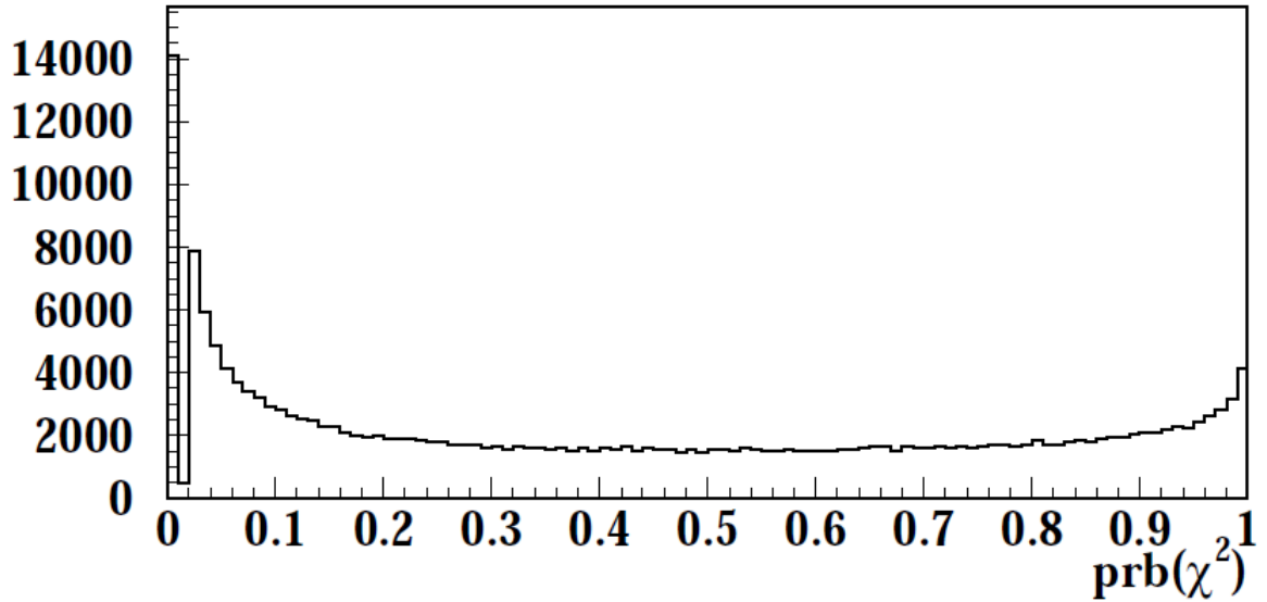
Figure 3.2: The distribution of the \chi^2 probability of track fitting by LEPS spectrometer.
