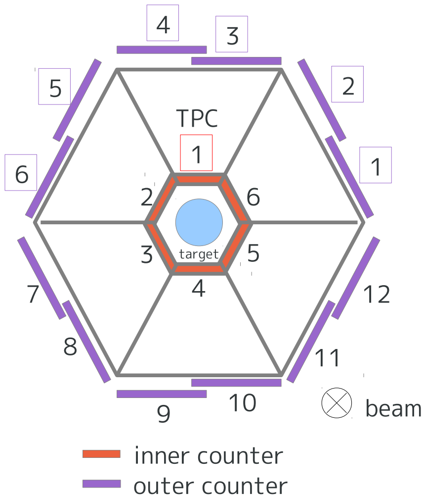
Figure 2.38: Logic of the 'Sector1' trigger. When inner counter 1 and at least one of outer counter 1-6 have coincident signals, 'Sector 1' trigger is generated.
