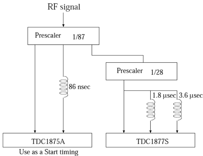
Figure 2.24: Circuit diagram for RF signals
