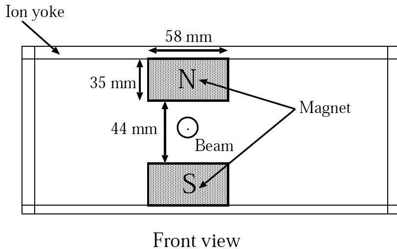
Figure 2.13: Structure of the sweep magnet.
