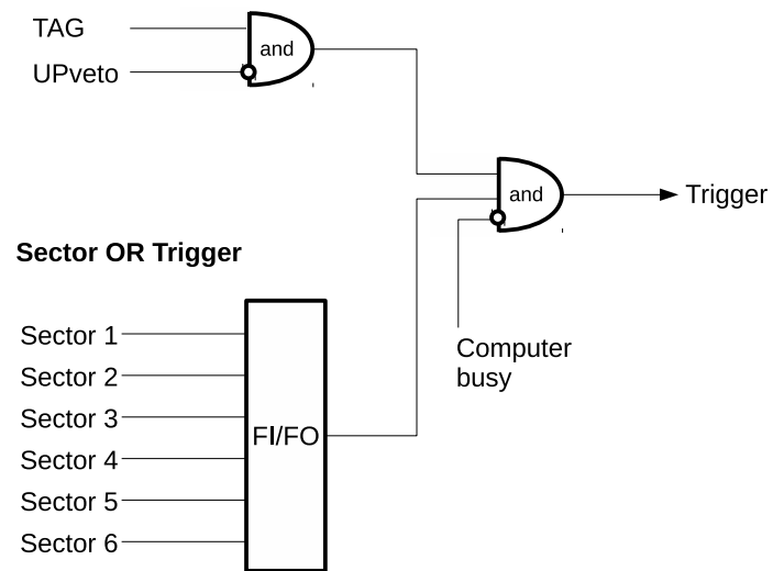
Figure 2.37: Diagram of the trigger logic for data taking.
