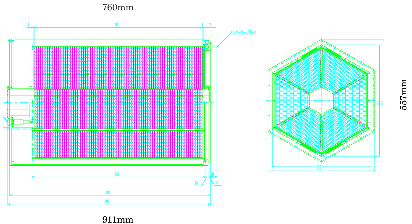
Figure 2.29: A schematic view of the Time Projection Chamber.
