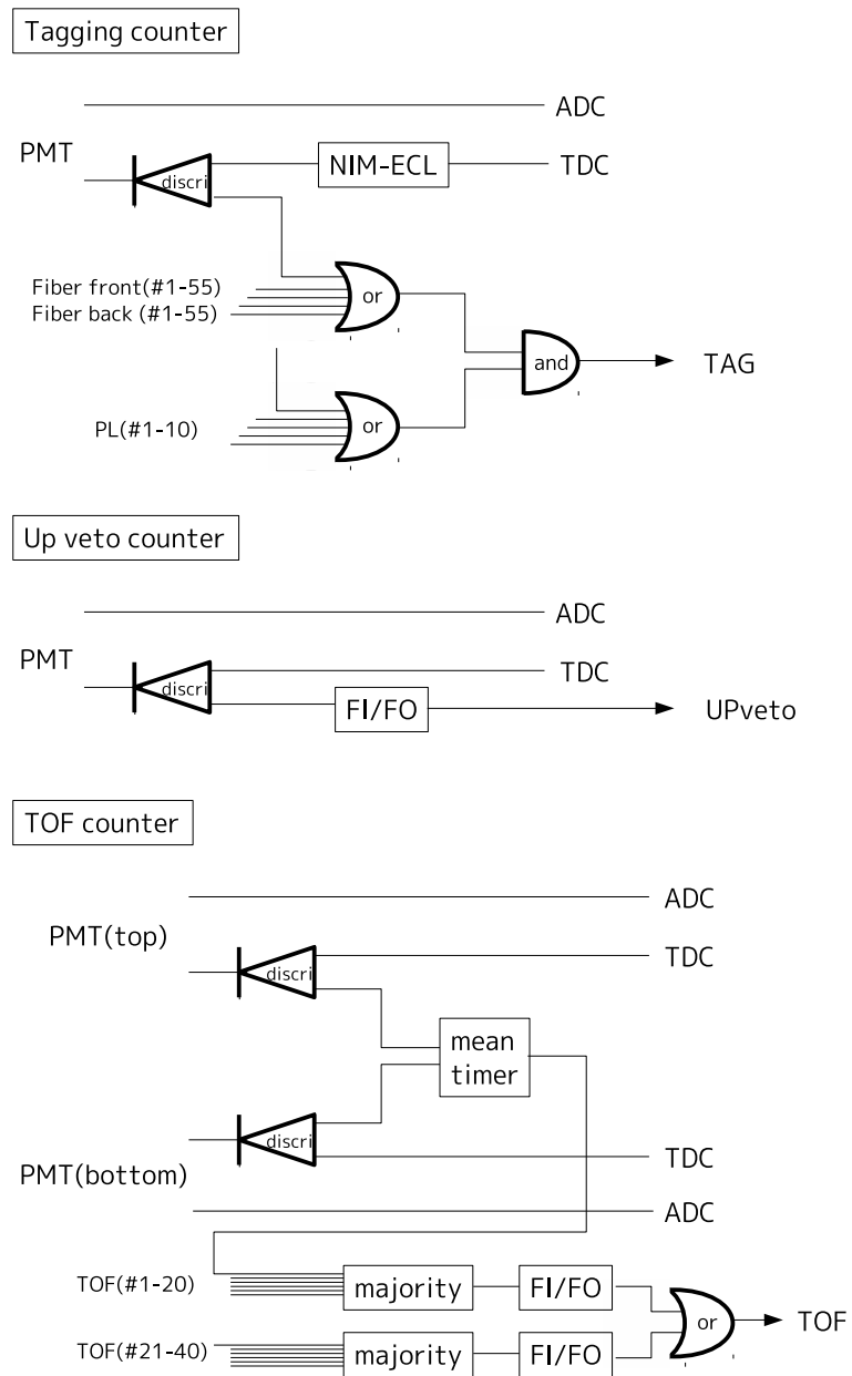
Figure 2.35: Diagram of the readout circuits for TAG, UPveto and TOF.
