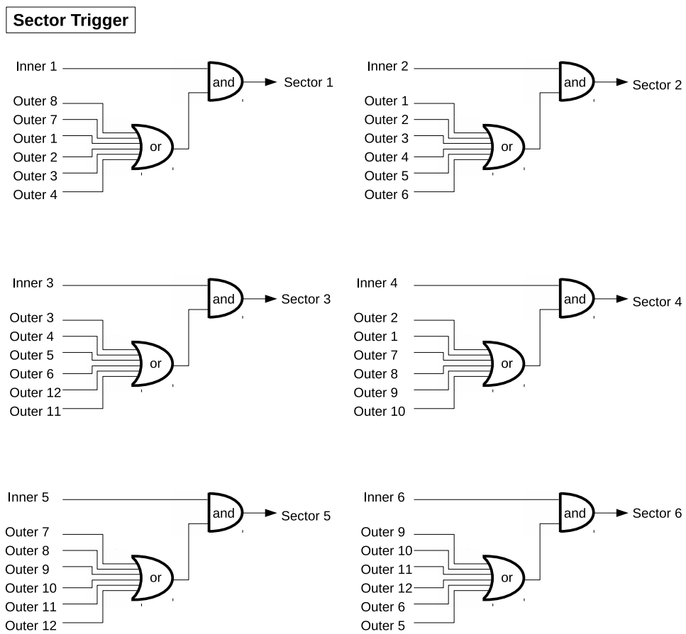
Figure 2.36: Diagram of the readout circuits for TPC inner and outer counters and Sector trigger logic.
